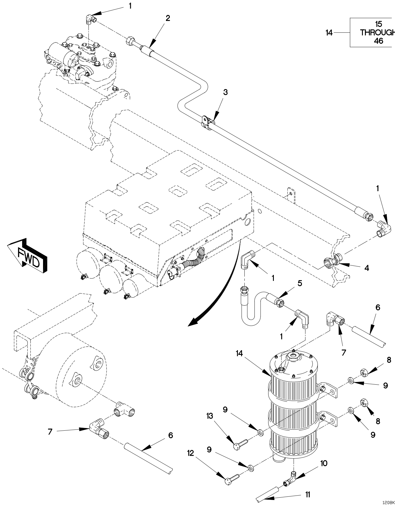
FIGURE 498. AIR DRYER, HOSES AND FITTINGS (SHEET 1 OF 2)
