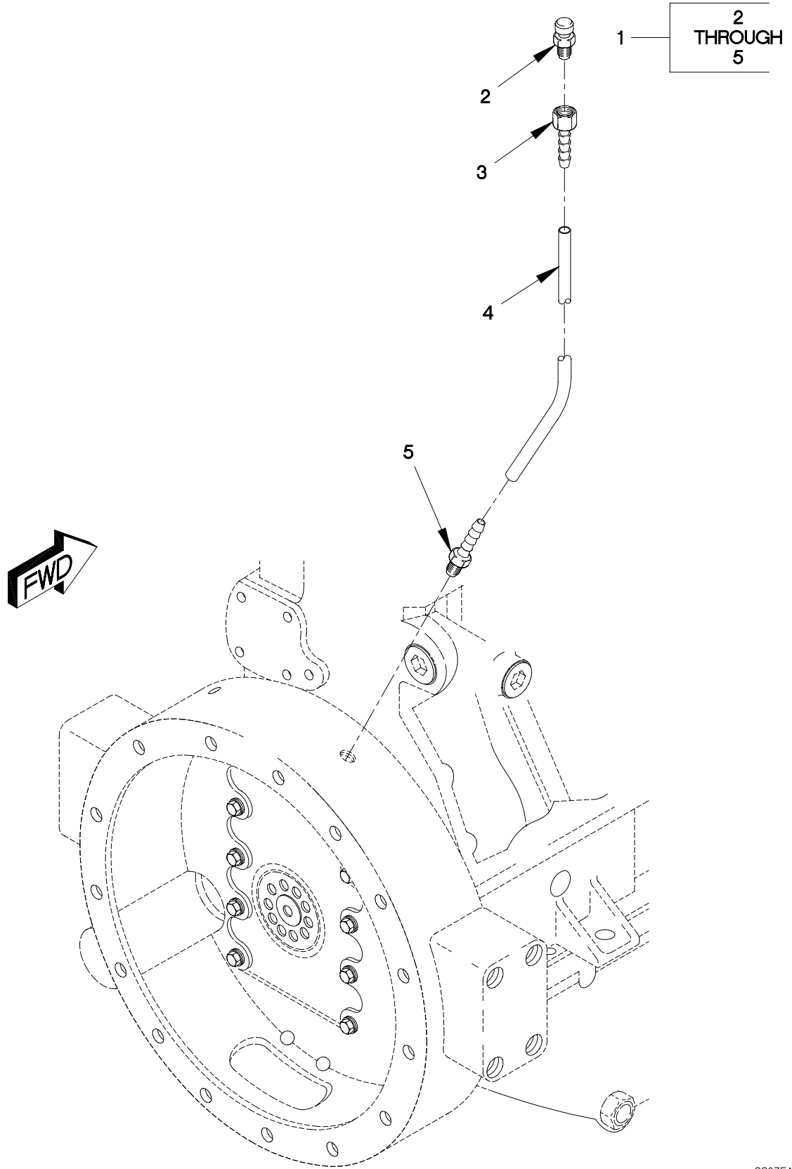
FIGURE 458. FLYWHEEL HOUSING VENT KIT
