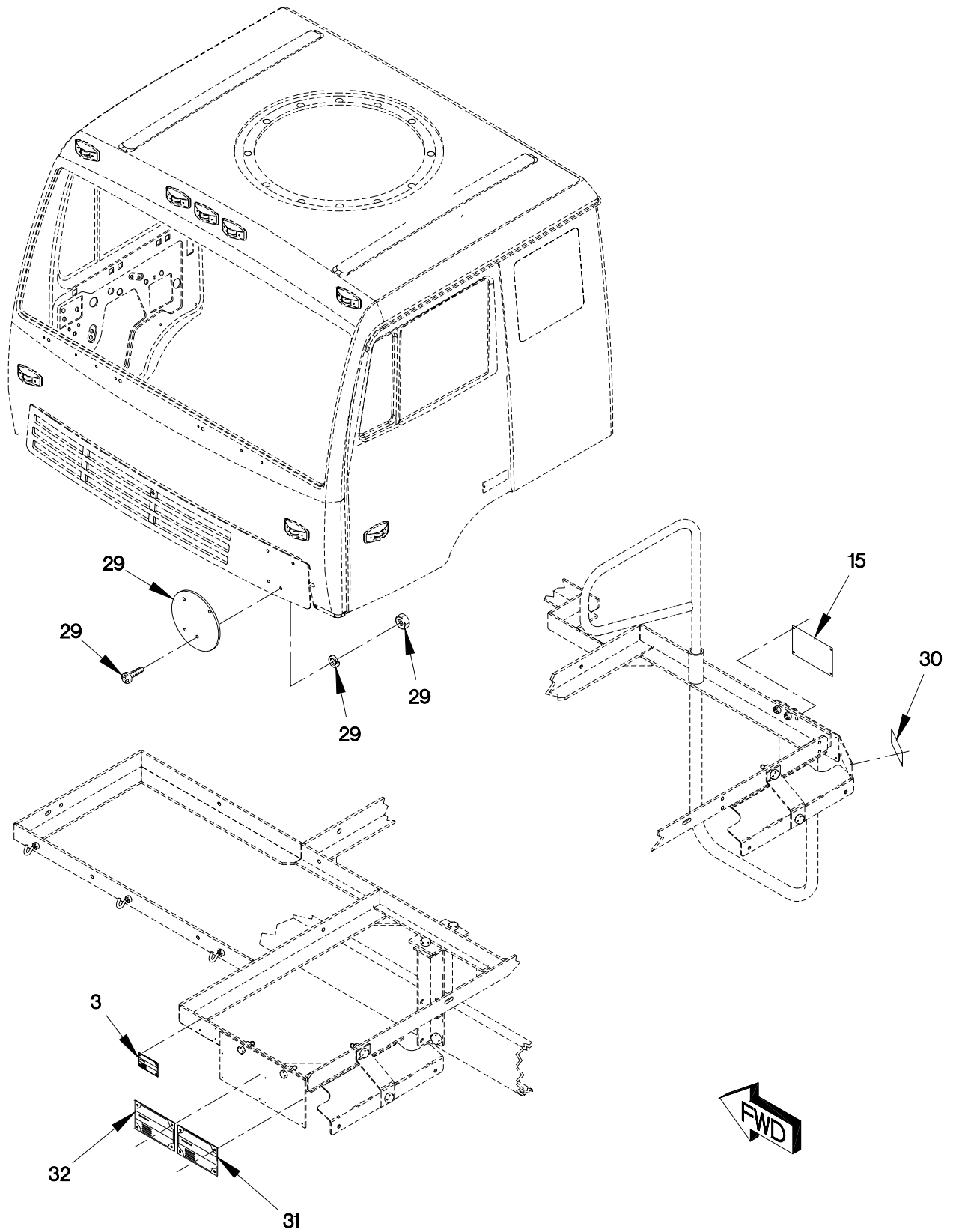
FIGURE 434. DATA AND IDENTIFICATION PLATES (SHEET 6 OF 6)
