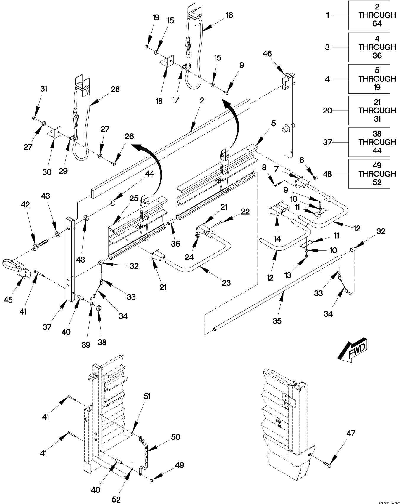
FIGURE 459. M1083 AND M1093 TROOPSEAT KIT (SHEET 1 OF 2)
