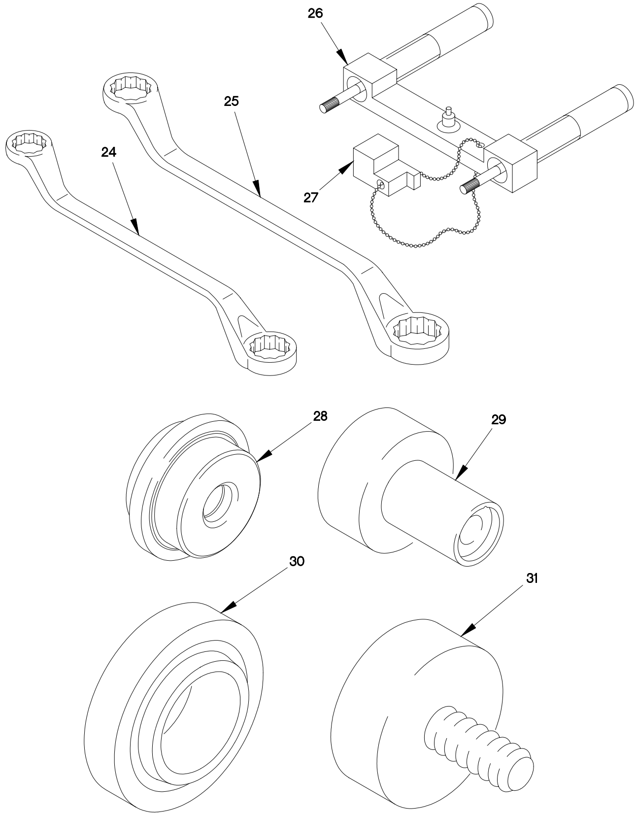
FIGURE 502. DIRECT SUPPORT MAINTENANCE SPECIAL TOOLS (SHEET 3 OF 3)
