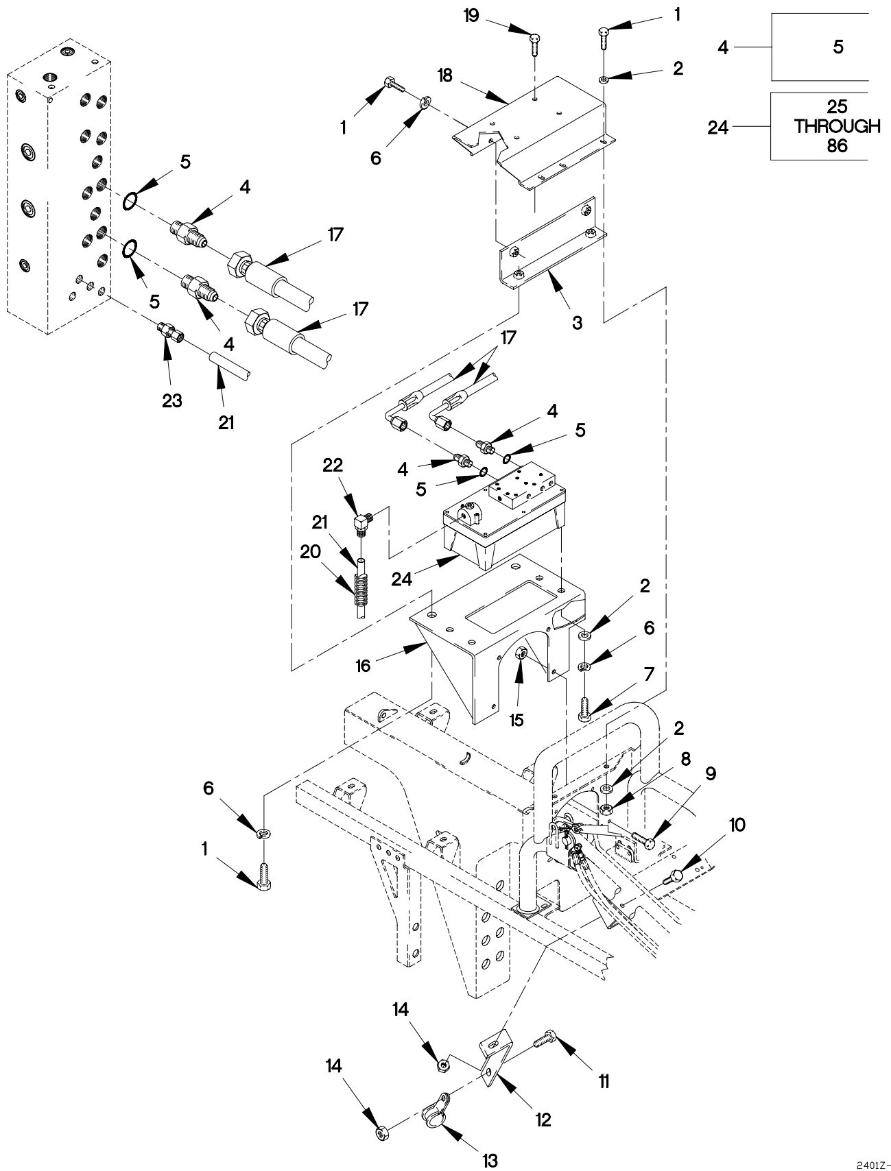
FIGURE 437. AIR/HYDRAULIC POWER UNIT, HOSES AND FITTINGS (SHEET 1 OF 2)
