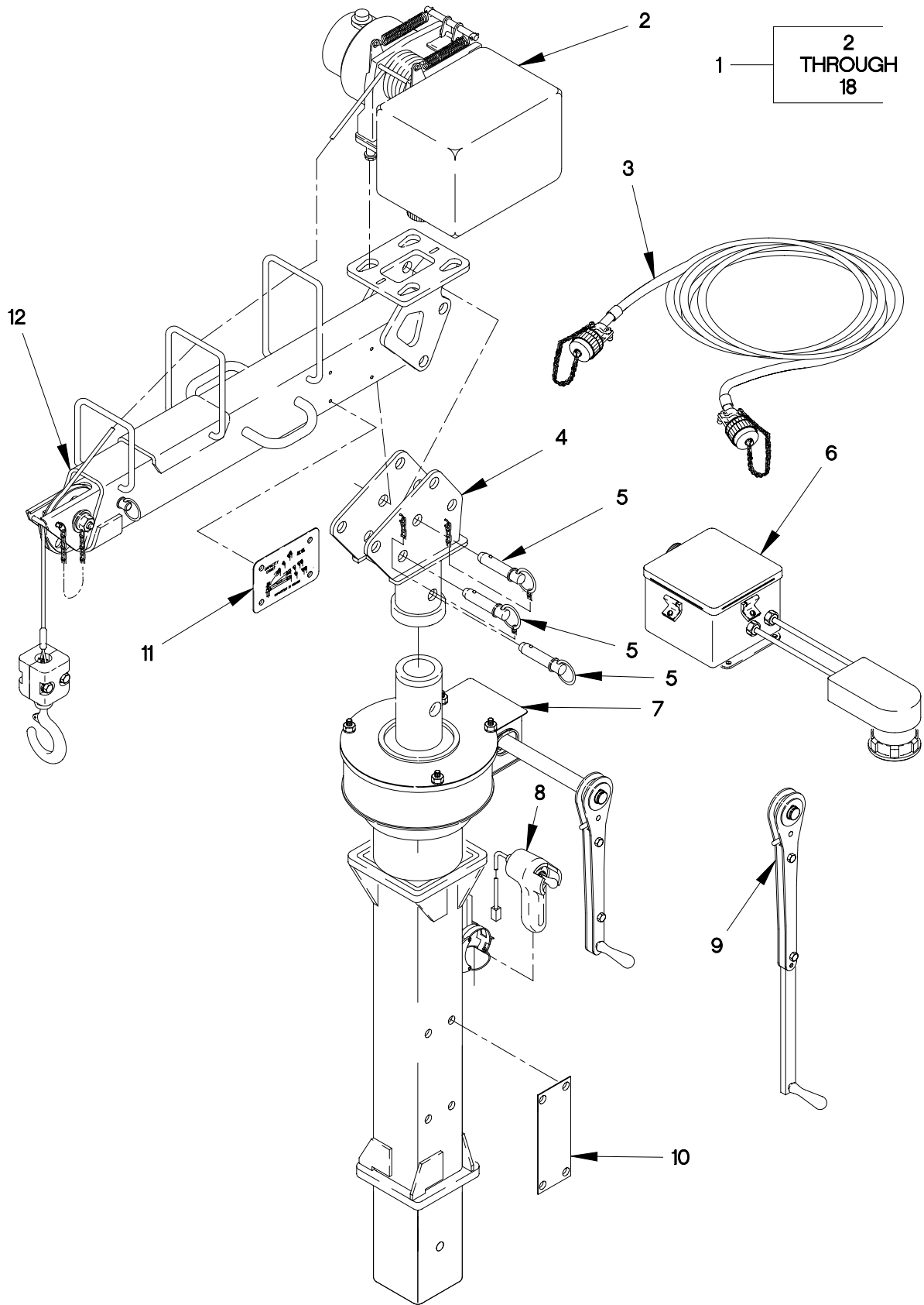
FIGURE 468. LIGHT MATERIAL HANDLING CRANE KIT (SHEET 1 OF 2)
