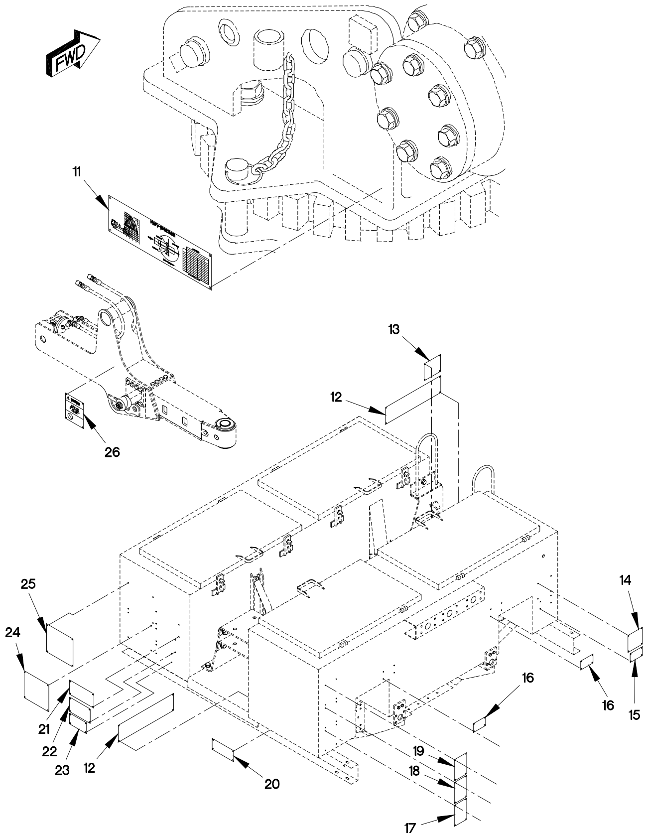
FIGURE 435. M1089 DECALS AND DATA PLATES (SHEET 2 OF 2)
