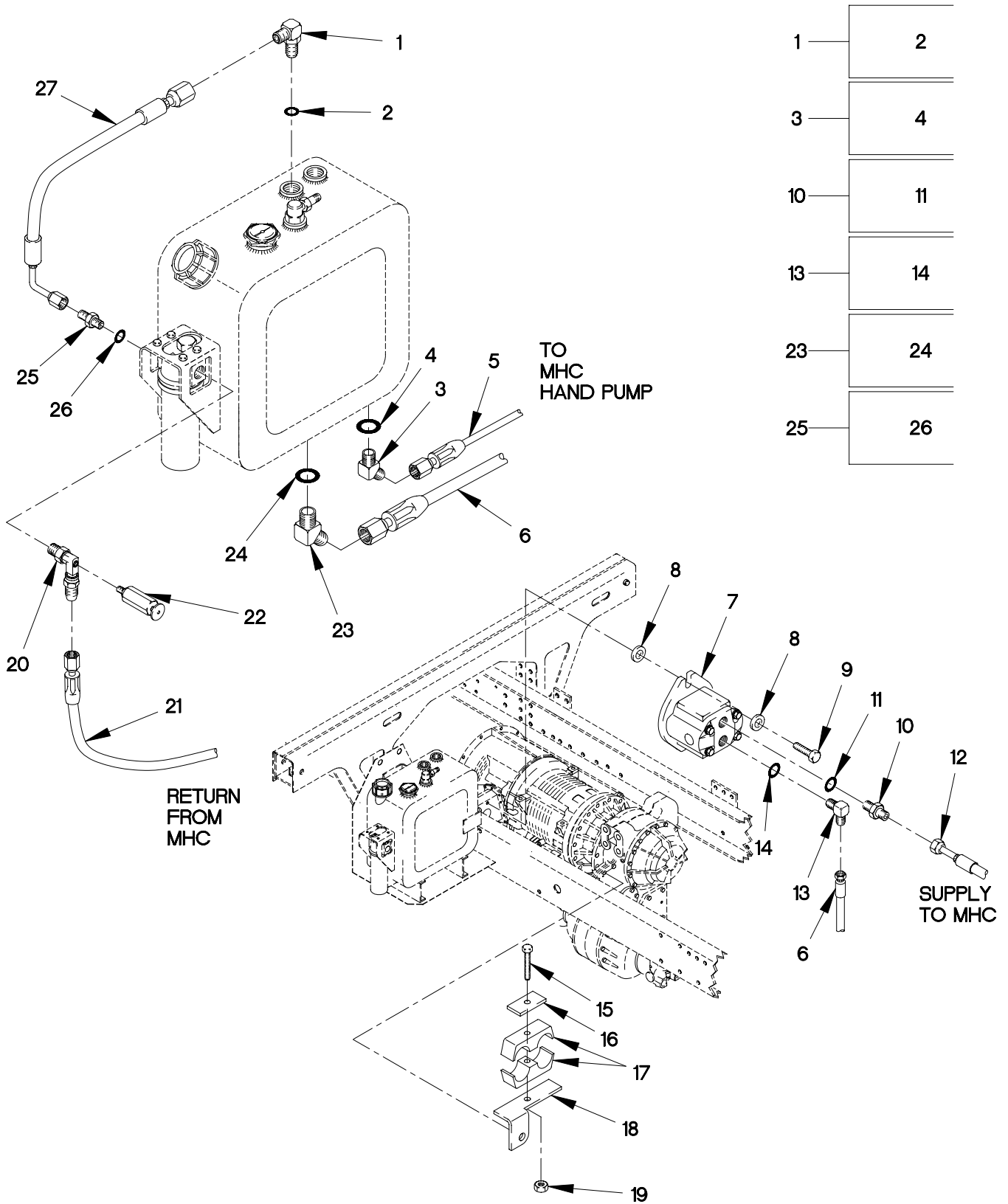
FIGURE 448. M1084 AND M1086 HYDRAULIC ROTARY PUMP, HOSES AND FITTINGS
