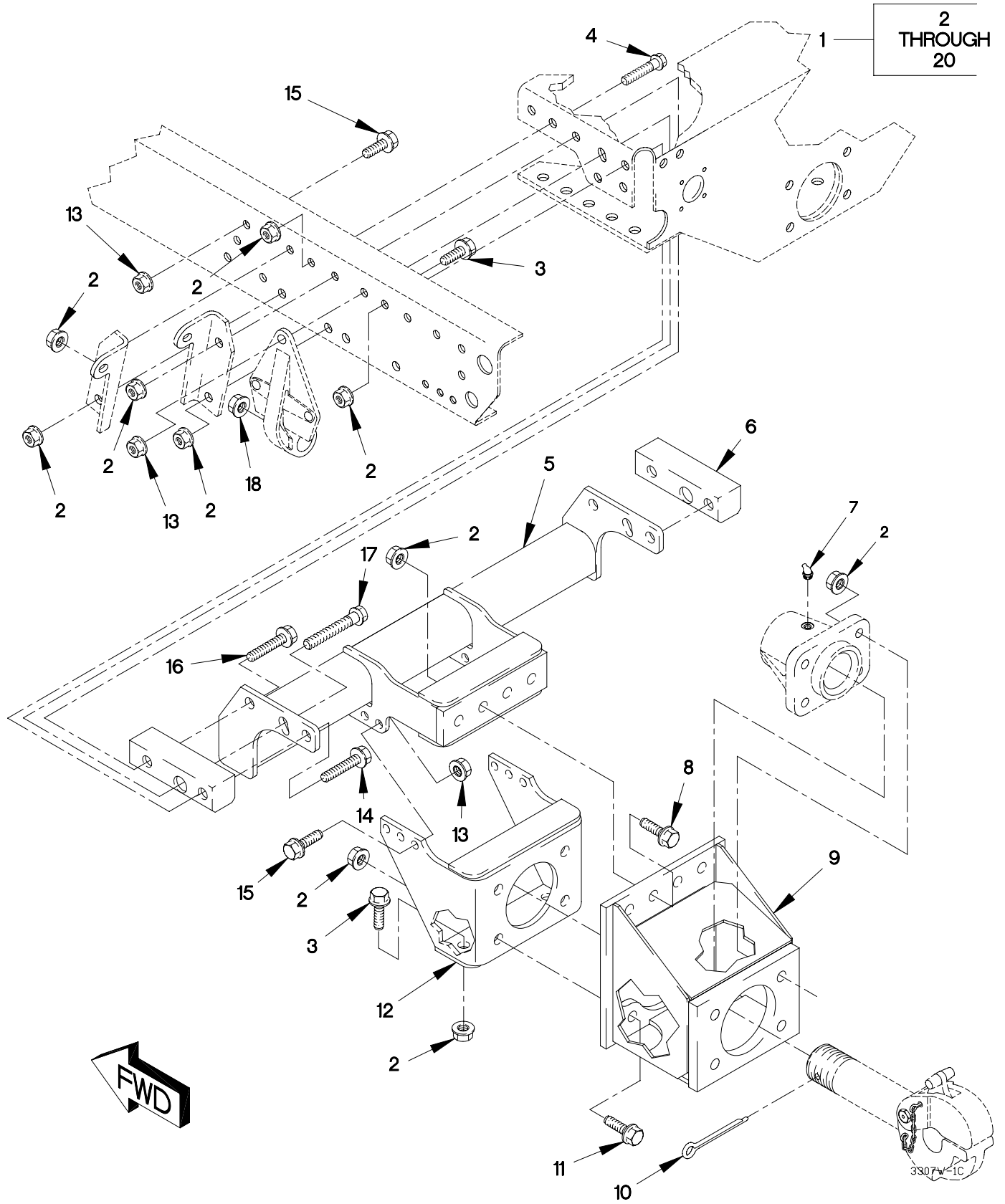
FIGURE 485. PINTLE HOOK EXTENSION KIT (SHEET 1 OF 2)
