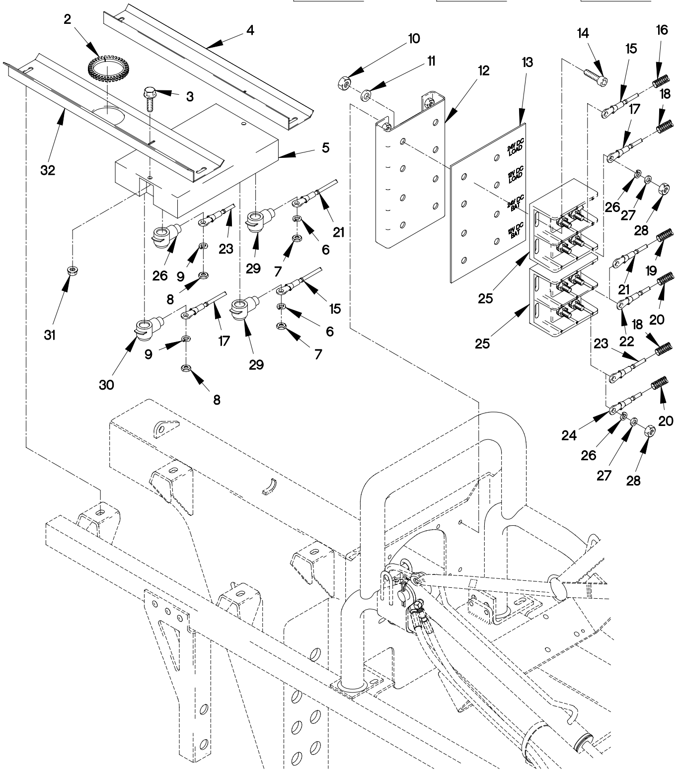
FIGURE 465. 200AMP POLARITY PROTECTION DEVICE, TERMINAL BLOCK, CABLES AND BRACKETS (SHEET 1 OF 2)
