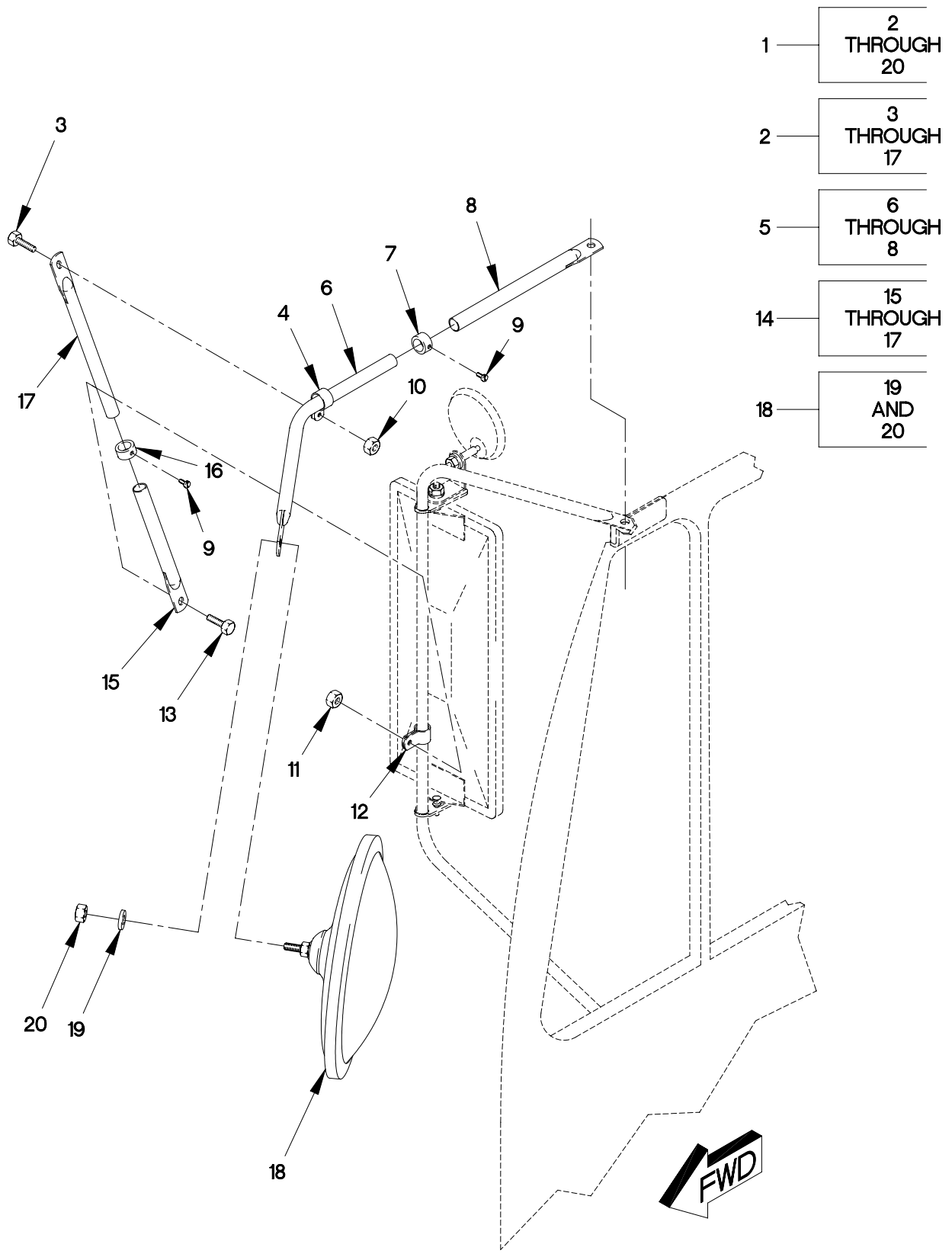
FIGURE 484. RIGHT CONVEX MIRROR KIT
