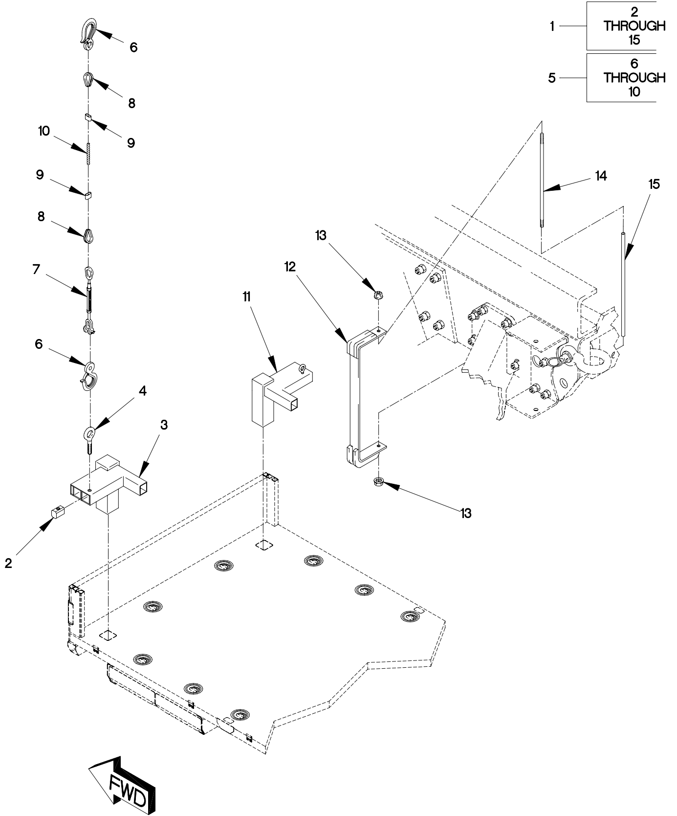
FIGURE 479. M1085 SHELTER TIEDOWN KIT
