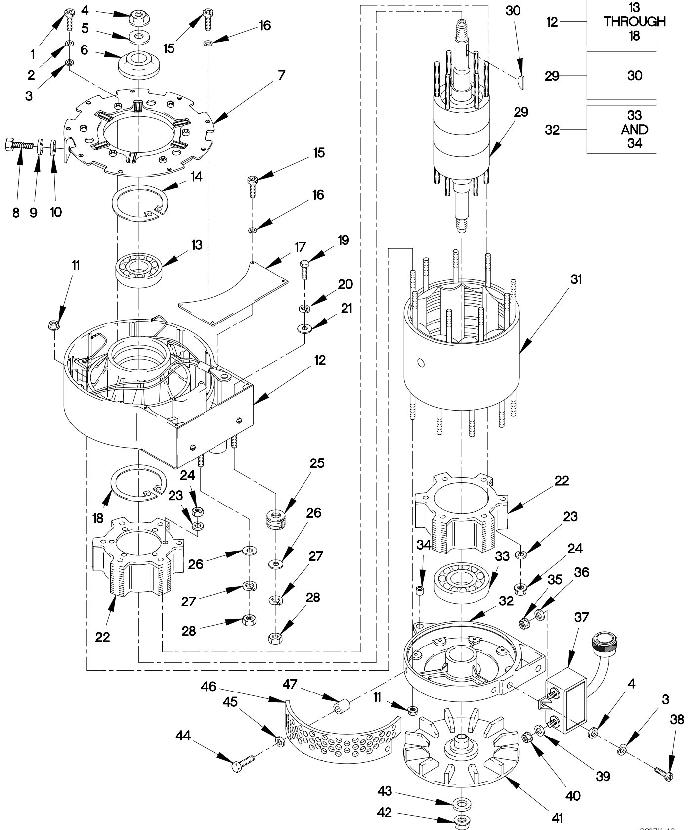
FIGURE 466. 200AMP ALTERNATOR AND REGULATOR
