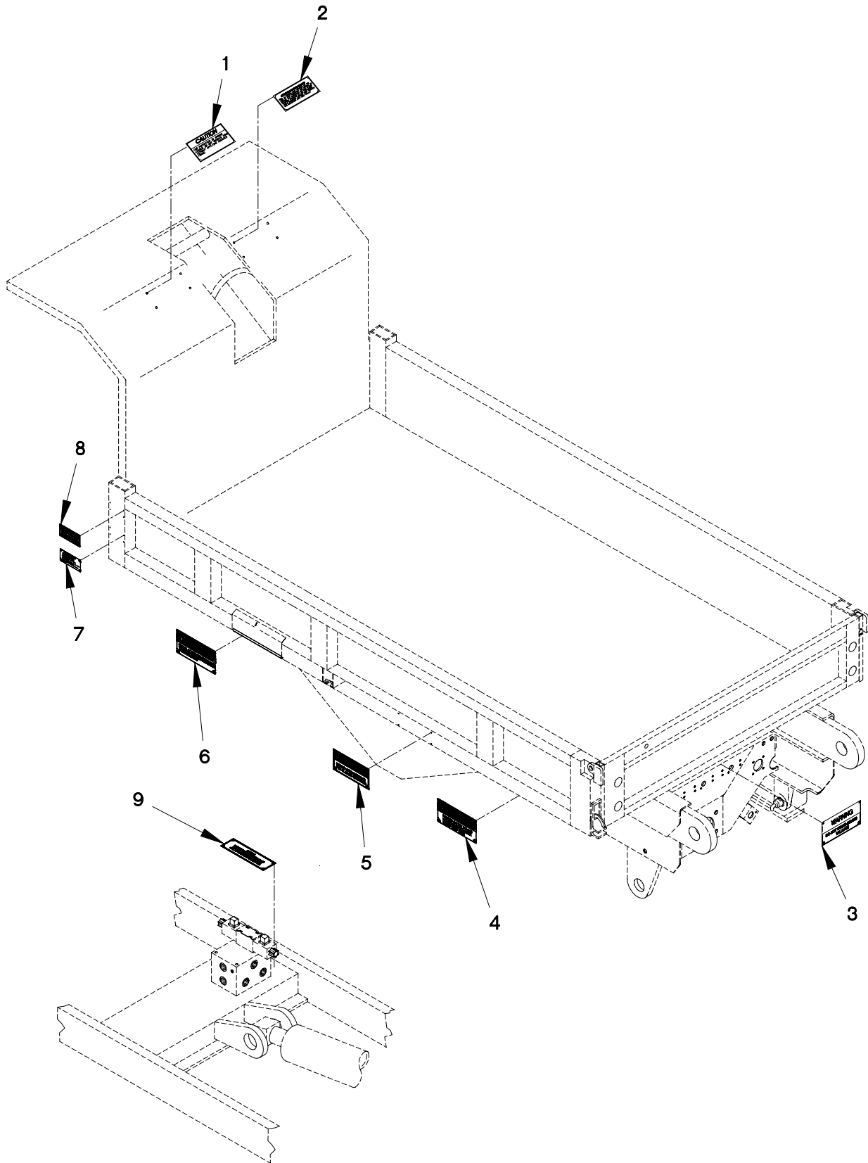
FIGURE 436. M1090 DATA AND IDENTIFICATION PLATES
