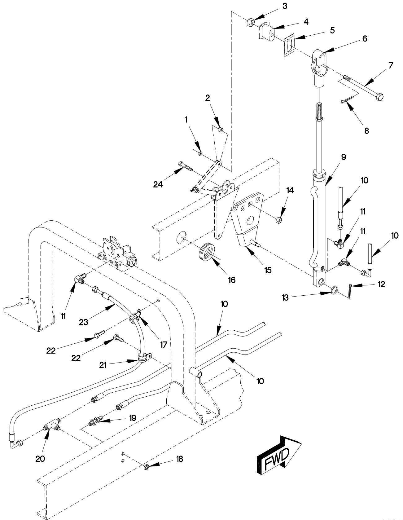
FIGURE 444. CAB HYDRAULIC CYLINDER, HOSES AND FITTINGS
