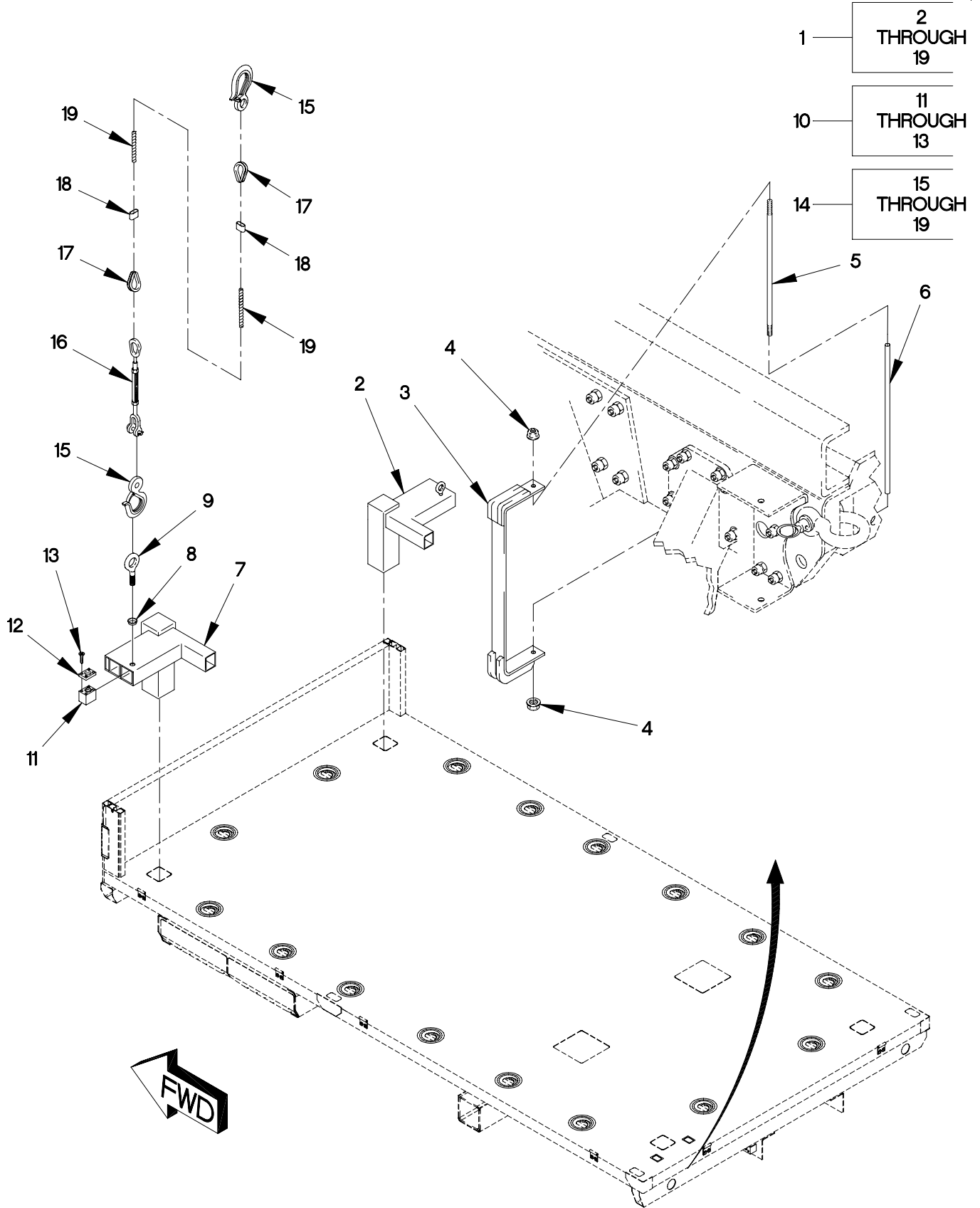
FIGURE 477. SHELTER TIE-DOWN KIT
