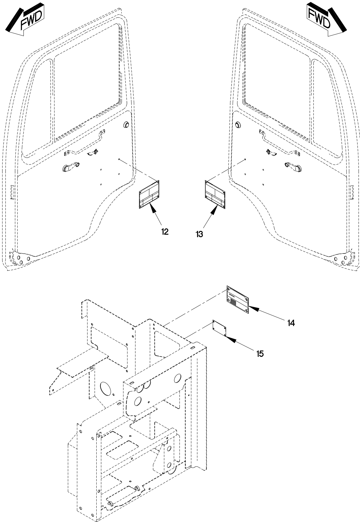
FIGURE 434. DATA AND IDENTIFICATION PLATES (SHEET 3 OF 6)
