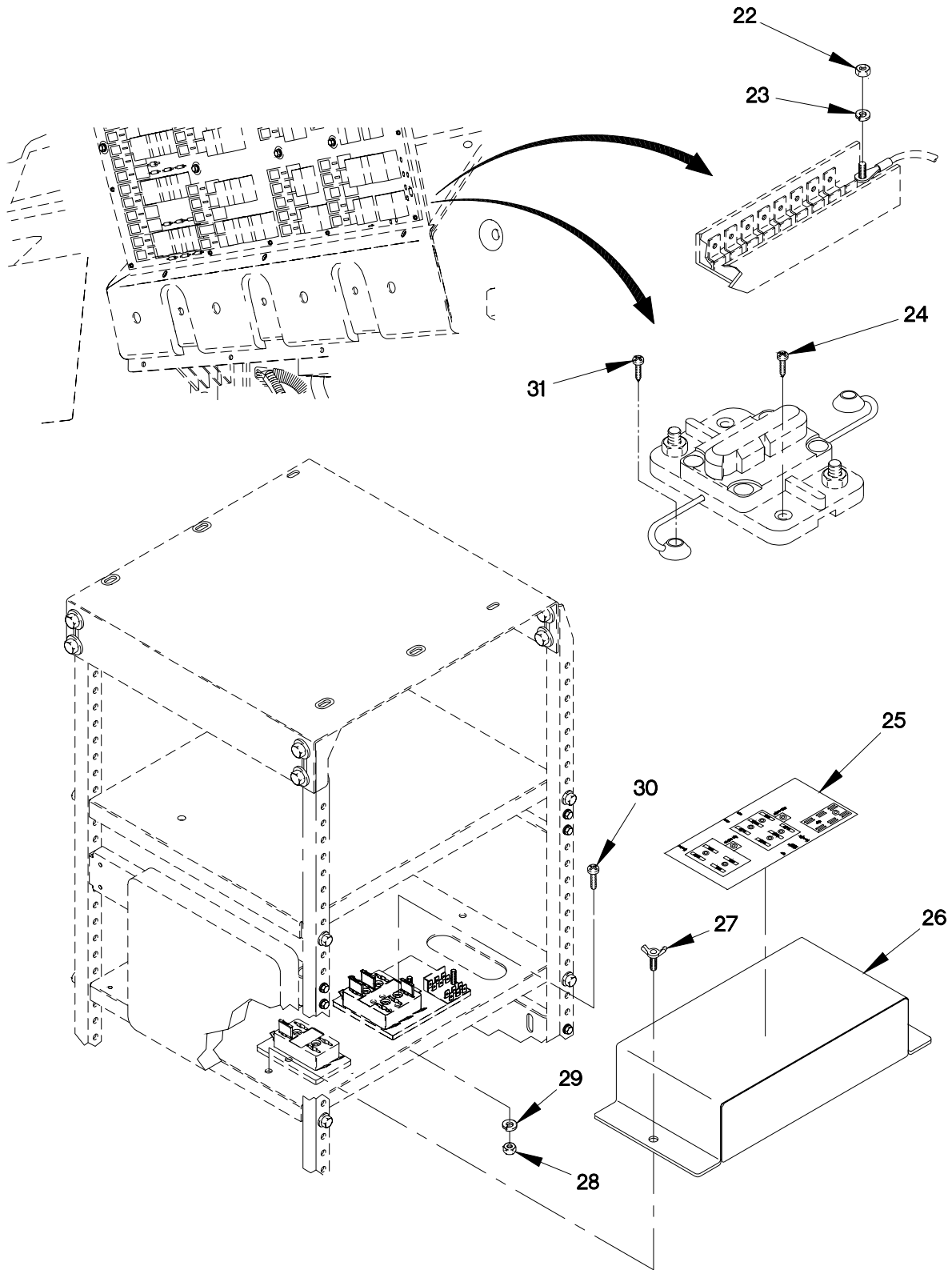
FIGURE 478. DIGITIZATION ELECTRICAL KIT (SHEET 2 OF 2)
