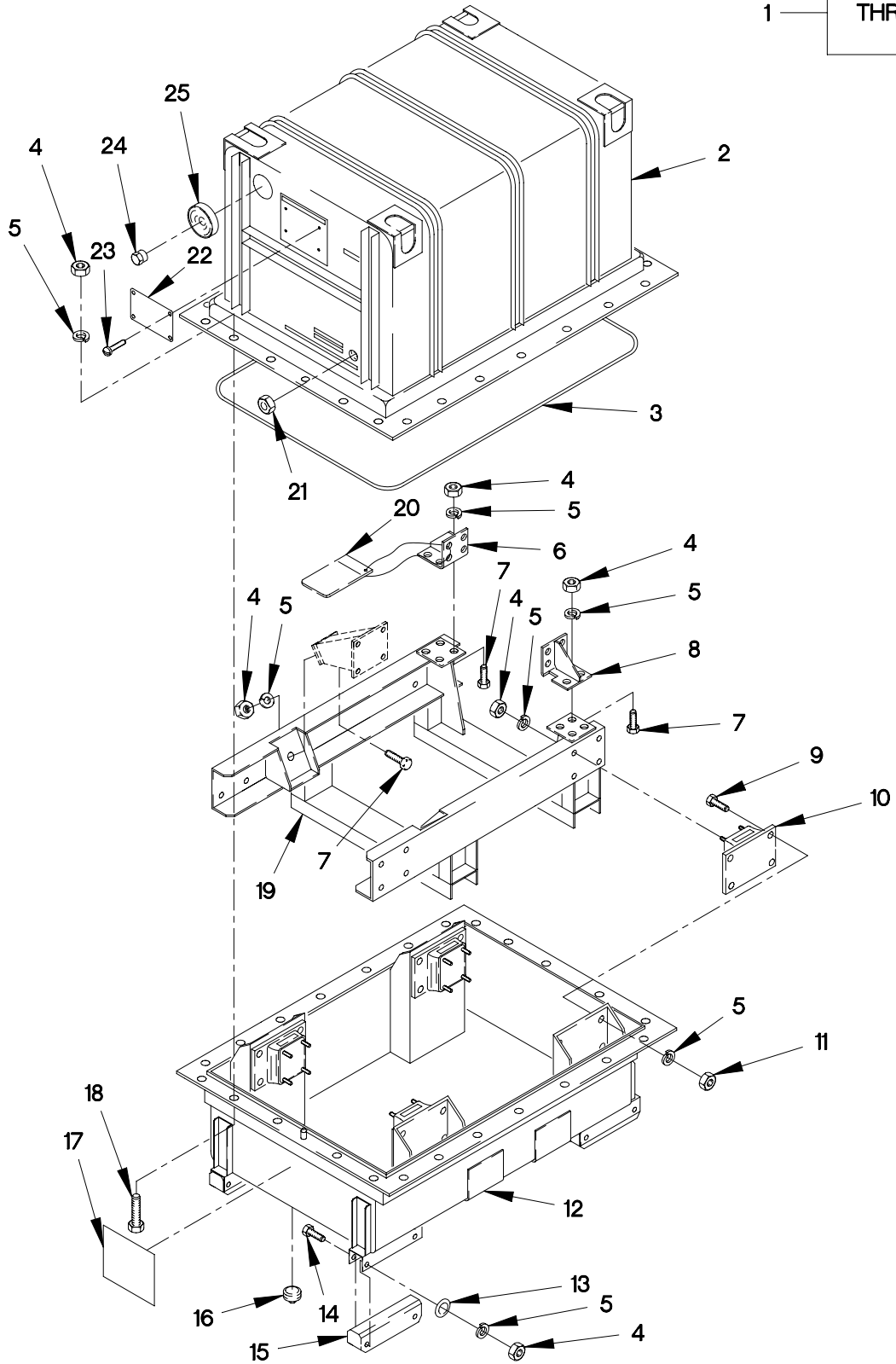
FIGURE 454. ENGINE CONTAINER
