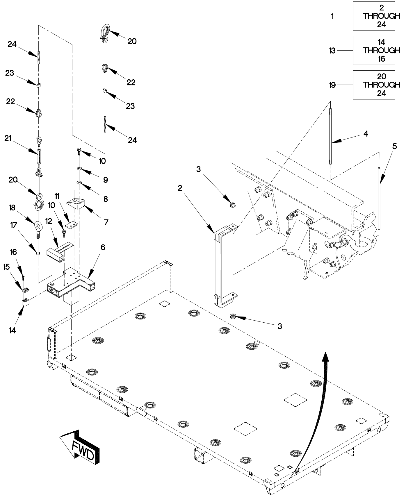
FIGURE 480. M1083 AND M1093 SHELTER TIEDOWN KIT
