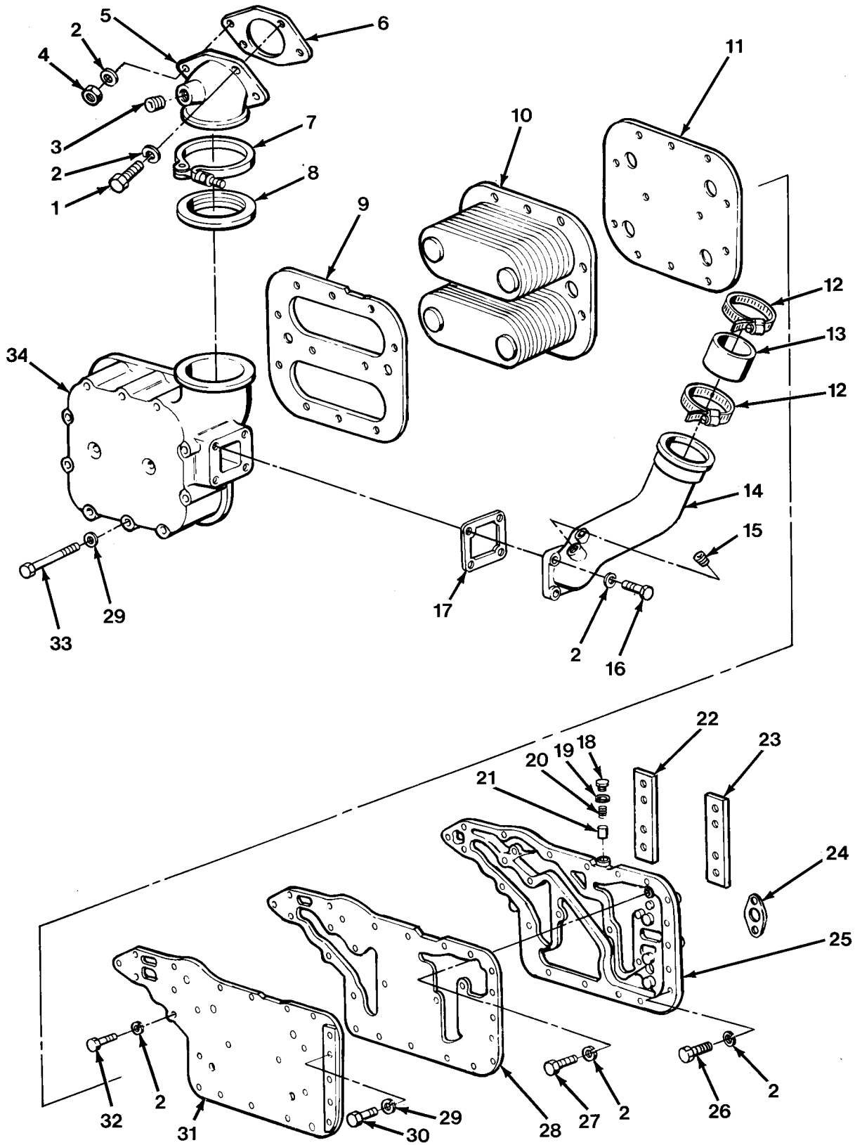
FIG.18 OIL COOLER
