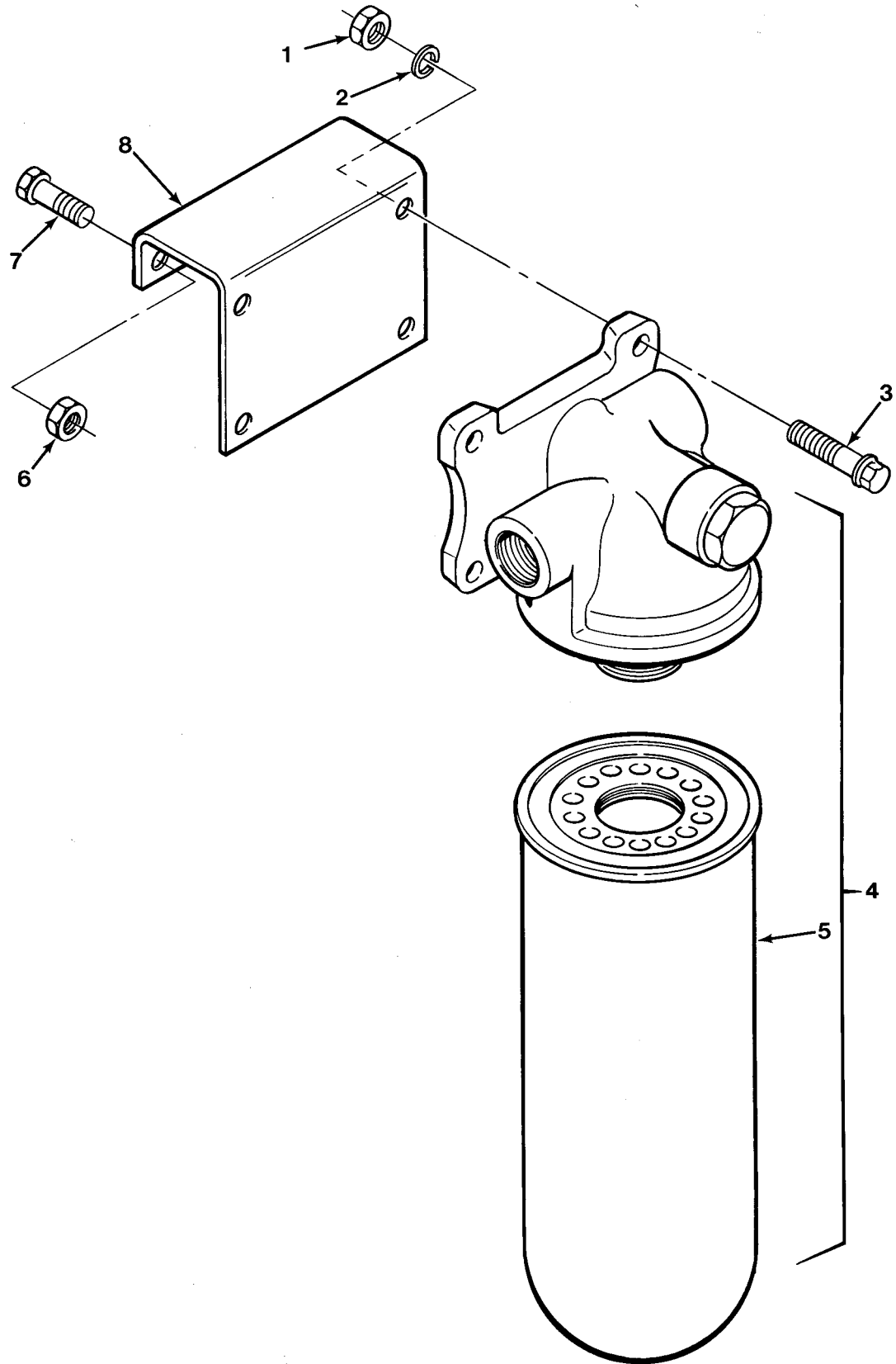
FIG.158 TRANSMISSION OIL FILTER
