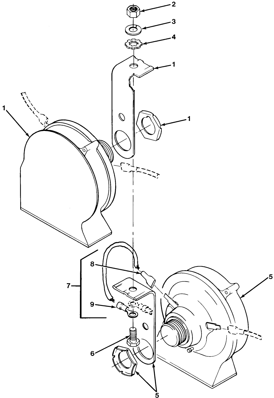
FIG.115 ELECTRIC HORN
