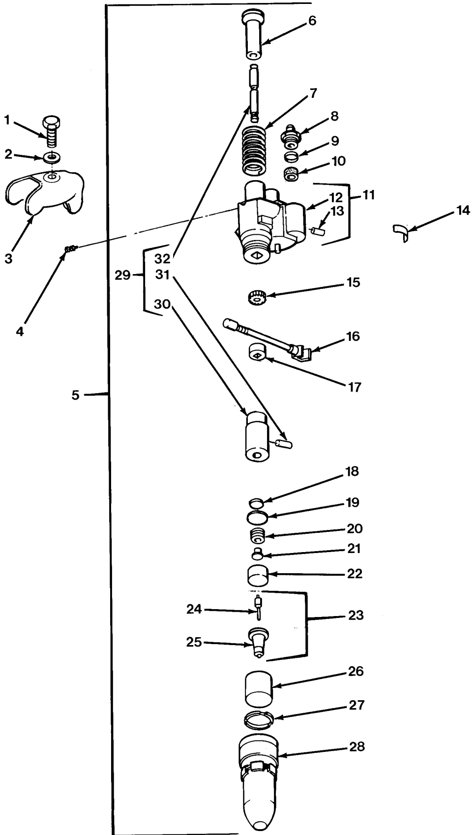
FIG.29 FUEL INJECTOR
